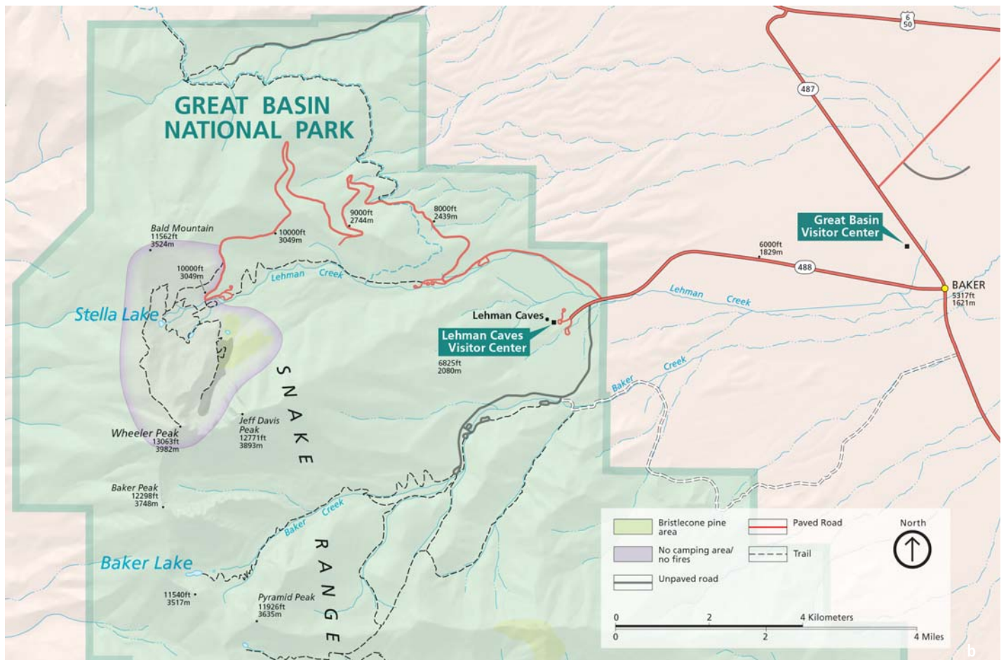
Figure 1. Lake cores were taken from Baker and Stella lakes, located in and near glacial cirques in Great Basin National Park. The park is situated in east-central Nevada.
