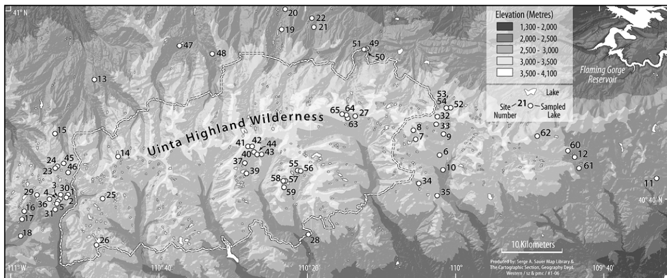
FIGURE 1. Location of study lakes in the Uinta Mountains, Utah. Numbers refer to lakes (see Table 1 for full lake names).
